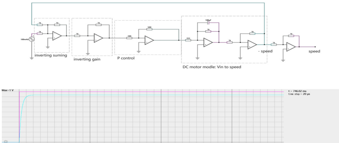
Fig. 9 Effect based on P control. (Photo/Picture credit: Original)
